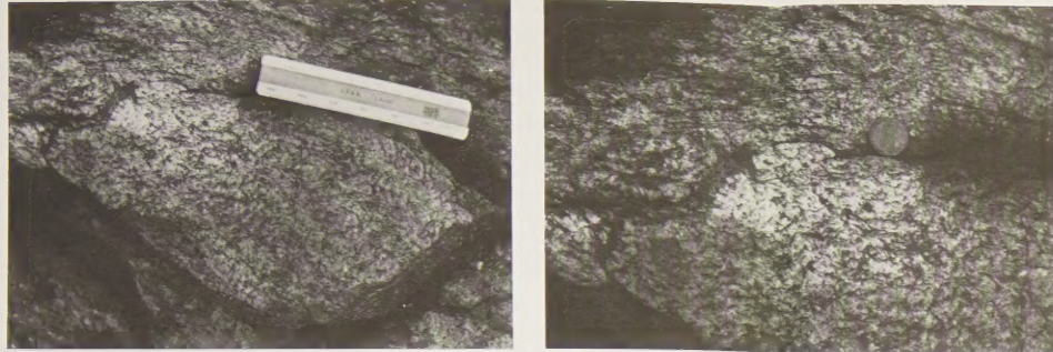
Figures 1 and 2. Outcrop photos of Phase One fabric at Loc. V13 (P1.2) viewed looking east. The phase one fabric is characterized by large, angular to rounded clasts of coarse-grained gneiss up to 30 cm in diameter. The clasts record only weak Paleozoic deformation compared to the well-foliated, fine-grained matrix that is composed of strongly deformed and altered gneiss. Major divisions on scale equal one inch (Fig. 1). Penny for scale (Fig. 2).
